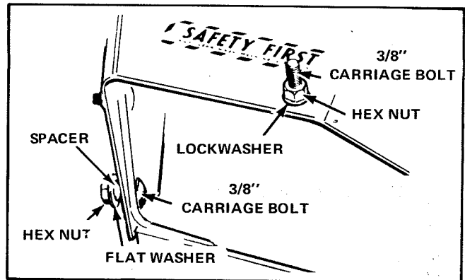
Figure 15. Preparing Mower Deck
